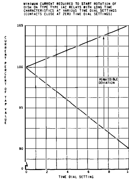
Fig. 4 Permissible Deviation of Current Required to Start Rotation of Disk
