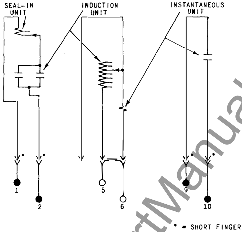
Fig. 1 Type IAC66C Relay, Internal Connections (Front View)
