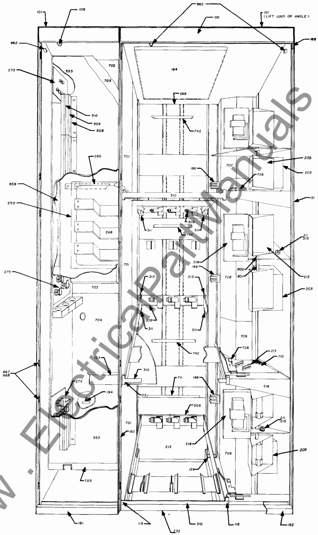
Three-high Construction
