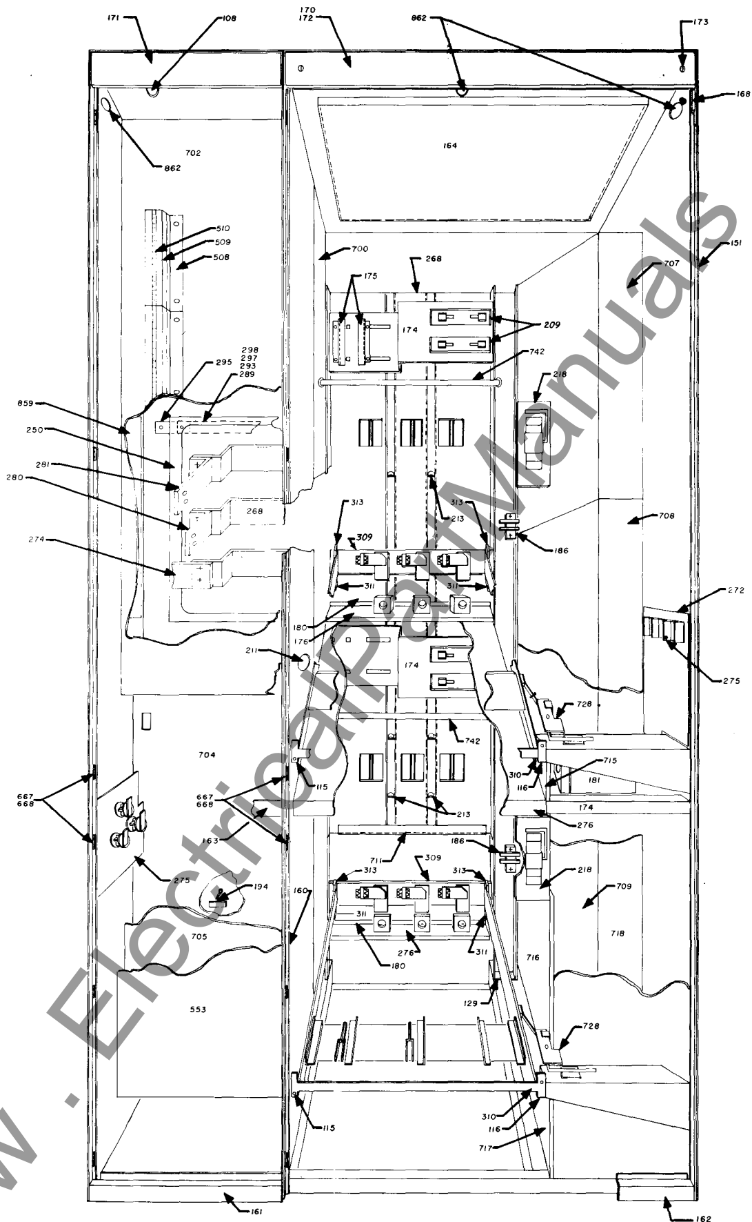
Two-high Construction
