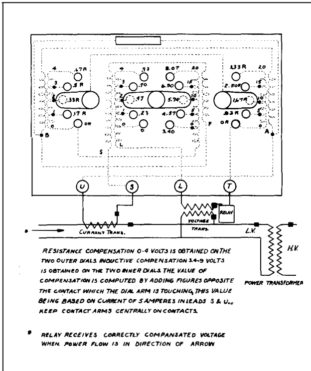
Fig. 9—Internal Connections of S#458551 Type KX Compensator.
