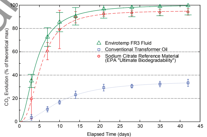
Aerobic Aquatic Biodegradation Graph EPA Test OPPTS 835.3100
